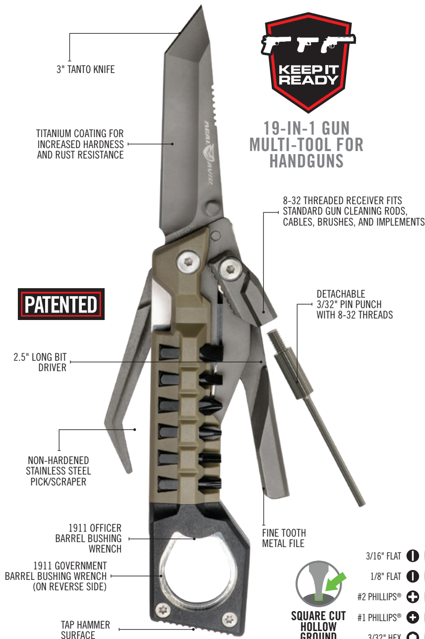
Disassemble guns with pin punch & integrated tap hammer
